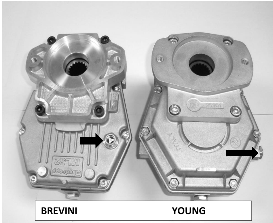
Figure 1—Identify the increaser by noting the location of the lubricant sight glass.
